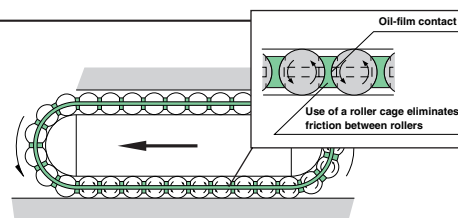
Caged Roller Structure
