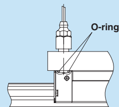
Method for using the greasing hole on the top face
