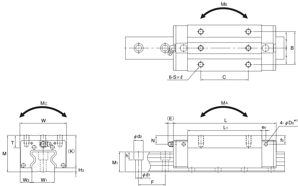
Models SRG25 to 65R/LR/LV
