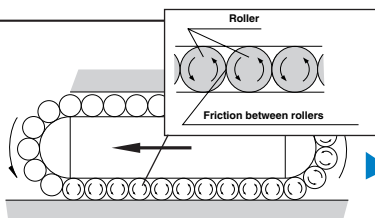
Conventional Structure
