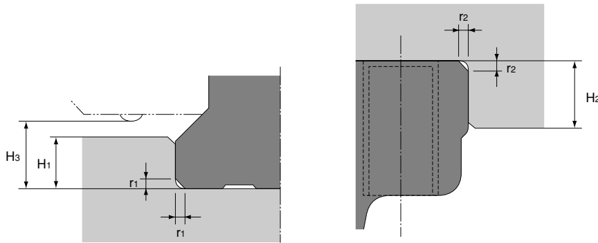
Shoulder for the LM rail
